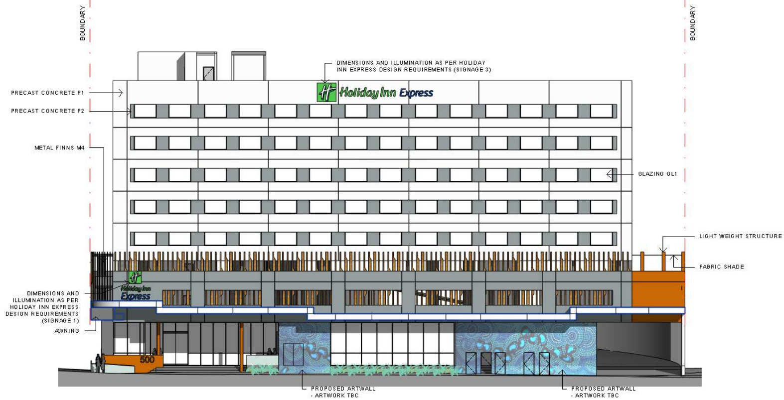
ELEVATION - PERFORATED METAL FINNS - 5 DIFFERENT PROFILES
